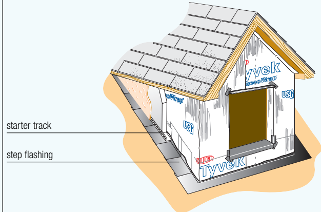
Typical Roof/Wall Drawer
