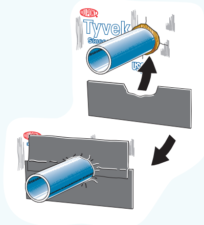
Typical Wall at Pipe/Penetration
