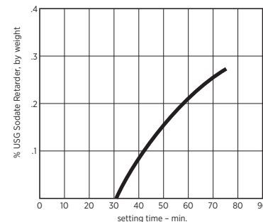
Fig. 8—Approximate retarding effect of USG Sodate Retarder on moulding, casting or pottery plasters.
