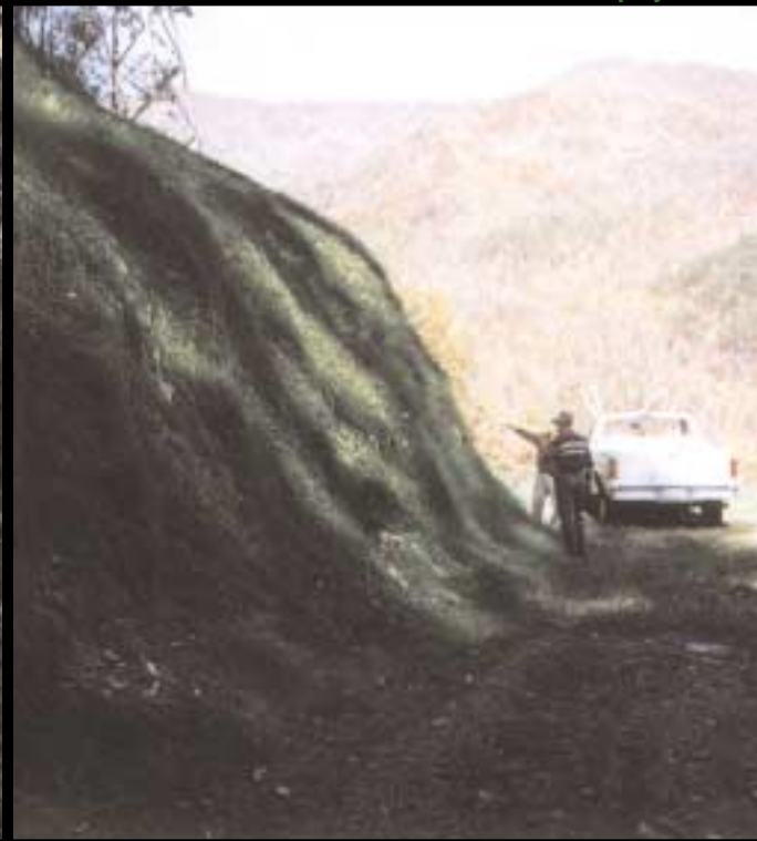
AIRTROL Geobinder helps prevent rill erosion on steep slopes, resulting in superior vegetation coverage.
