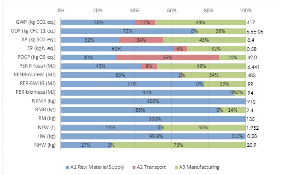
Figure 4: EPD Results by Information Module – 1 MSF of 5/8" GMP – % Basis
