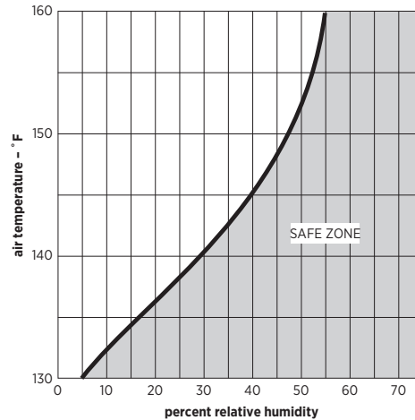
Fig. 3—Minimum relative humidity at temperature to prevent calcination of gypsum casts.
