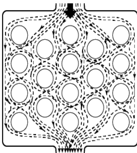
Fig. 2—Air-flow pattern for proper circulation in drying chamber.
