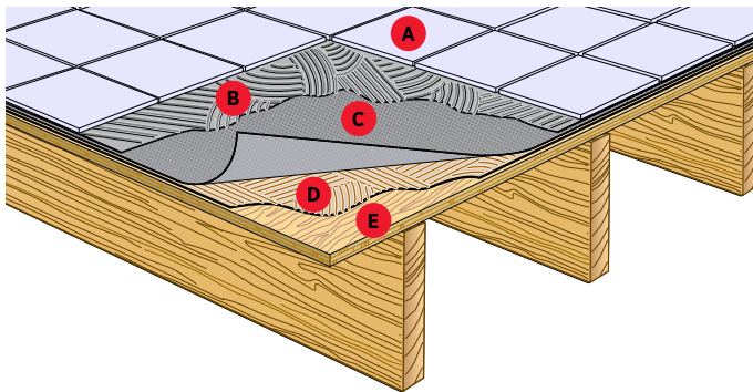
Wood Subfloor
