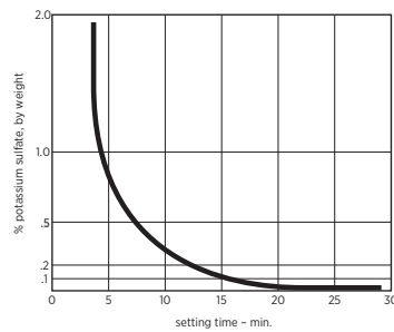
Fig. 5—Approximate accelerating effect of potassium sulfate on moulding, casting or pottery plasters.
