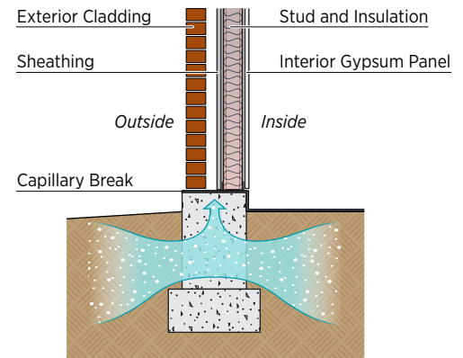
Capillary Suction (Controlled by means of a capillary break)
