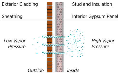
Outward Vapor Flow by Diffusion (Controlled by means of a vapor retarder)
